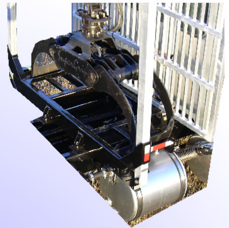
Front Bunk with Bucket Carrier
